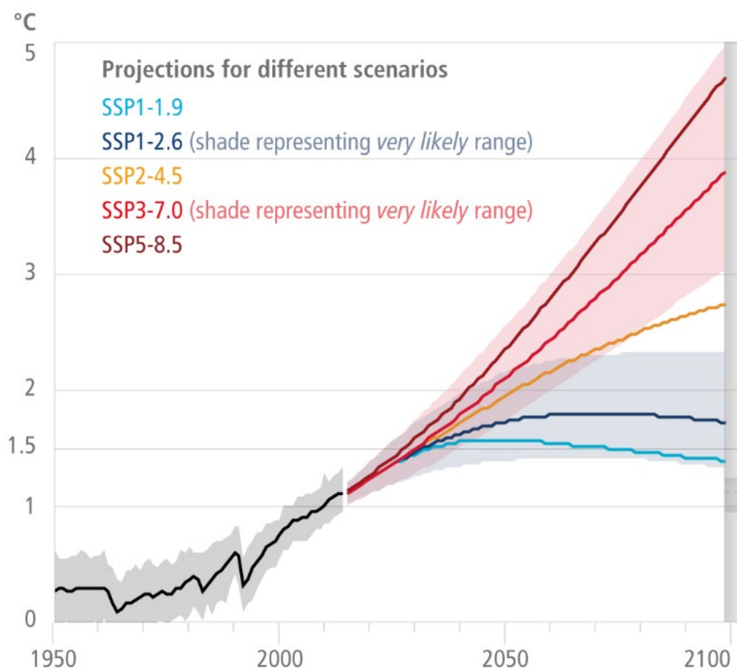
Figure 2. Projected changes in global surface temperature (°C) compared to 1850-1900 under five illustrative climate scenarios: very low emissions (SSP1-1.9), low emissions (SSP1-2.6), medium emissions (SSP2-4.5), high emissions (SSP3-7.0) and very high emissions scenario (SSP5-8.5). Source: IPCC Sixth Assessment Report, Working Group II, Technical Summary
