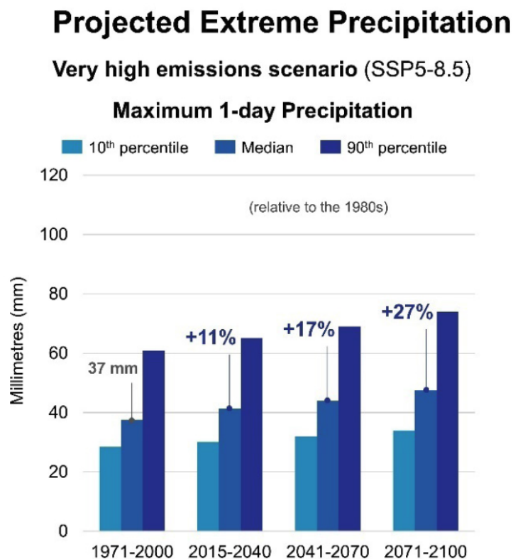
Figure 11. Projected maximum one-day precipitation under the very high emissions scenario (SSP5-8.5), with percentage differences in median values compared to 1971-2000 (modelled historical).
