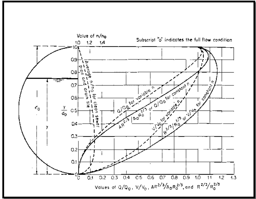
Figure 4: Hydraulic elements graph for circular pipe
