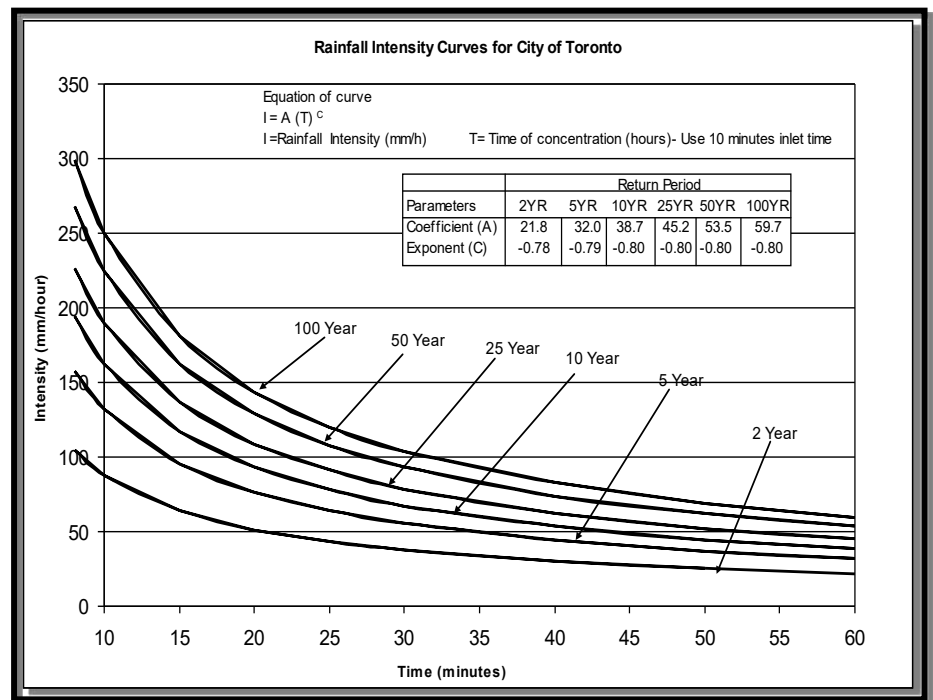
Figure 5: Rainfall intensity curves for City of Toronto
