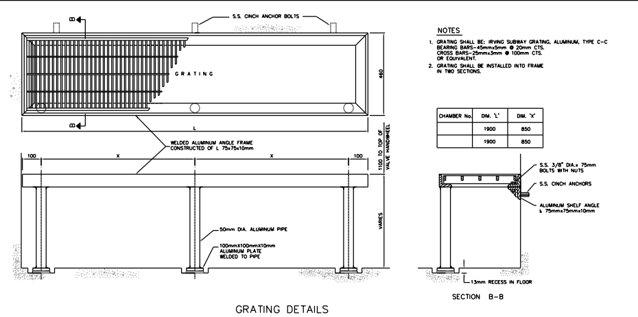
GRATING DETAILS
