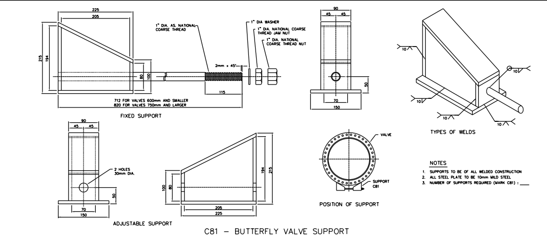
C81 – BUTTERFLY VALVE SUPPORT
