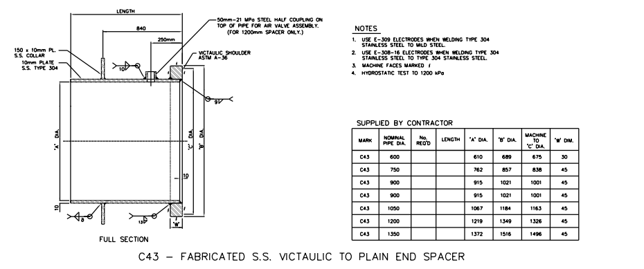
C43 – FABRICATED S.S. VICTAULIC TO PLAIN END SPACER
