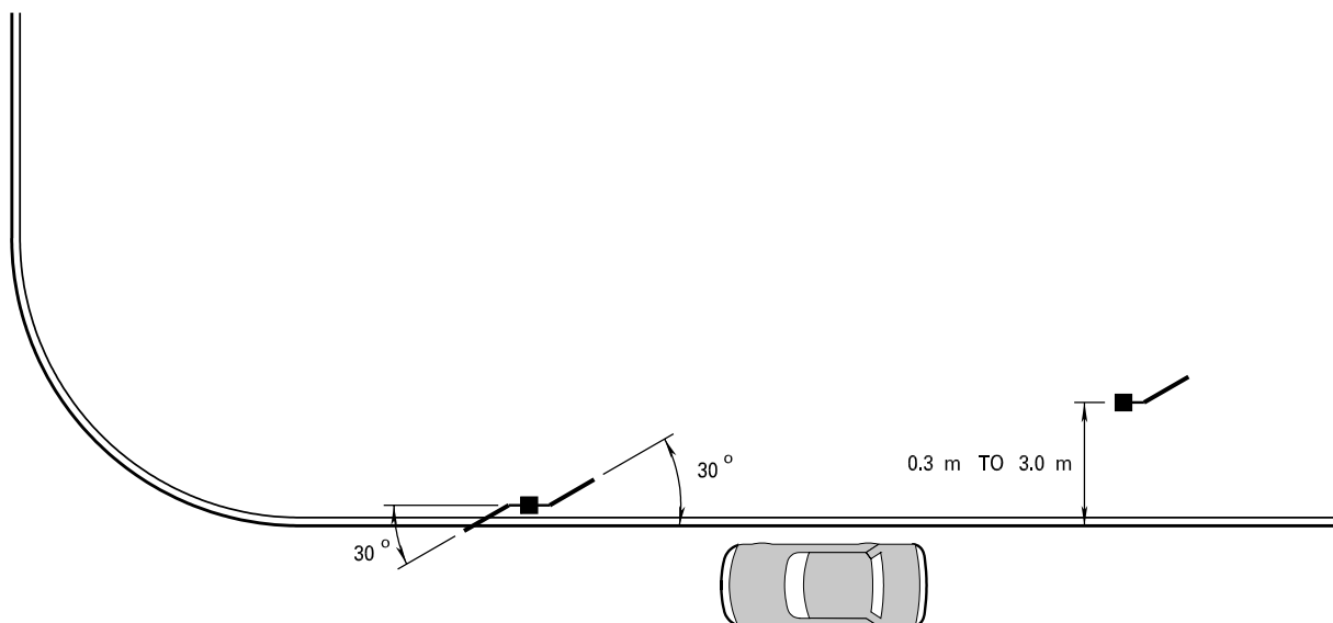
PLAN VIEW OF GENERAL LOCATION OF PARKING SIGNS
